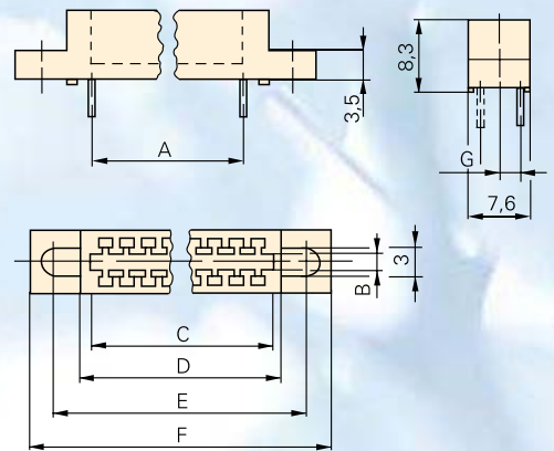
With flange
