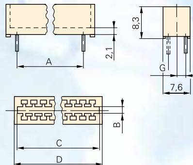
Without flange
